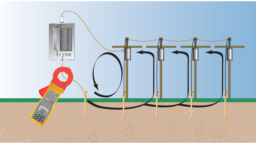
Test current paths in the stakeless method using 1630-2 FC Earth Ground Clamp.
